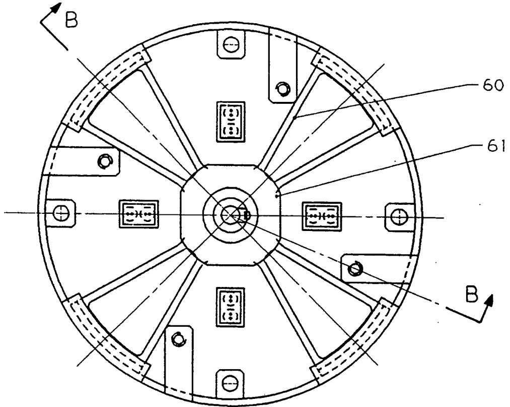
SECTION C-C - FIG 7
